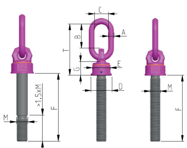
Pic. 7: VWBG-Vario with continuous thread
