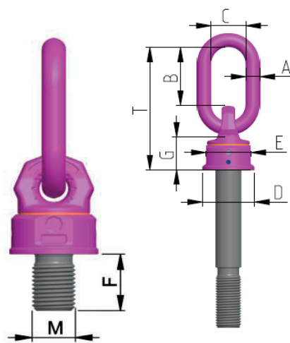
Pic. 6: VWBG-Vario with shaft
